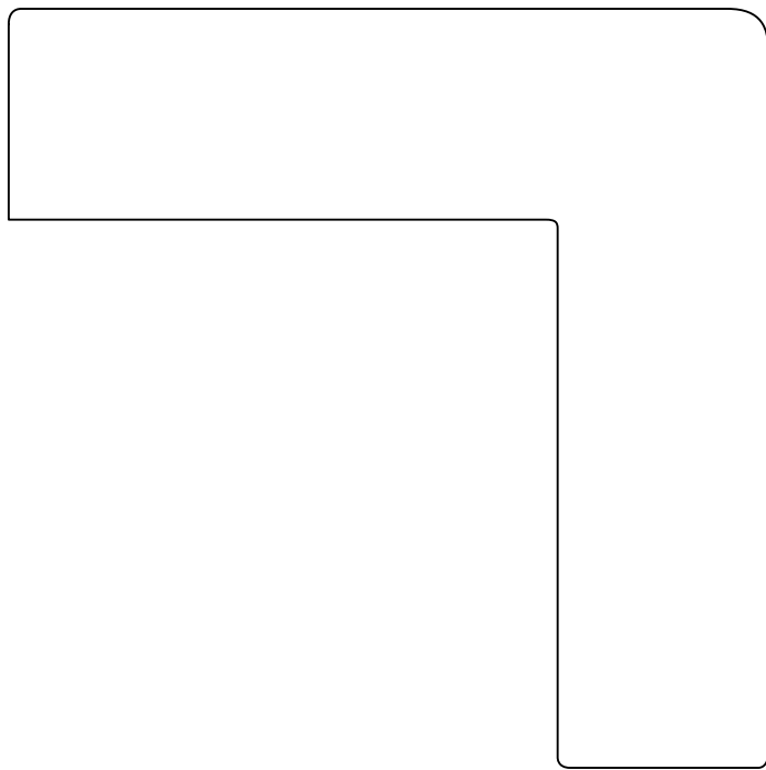
CB544PVC 1" x 3-1/2"
