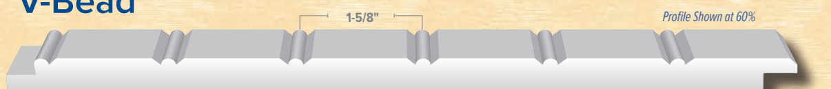
1-5/8" V-BEAD (9.6" FACE) 1 LINEAL FT = .80 SQ FT – ORDER IN 4 PIECE INCREMENTS
