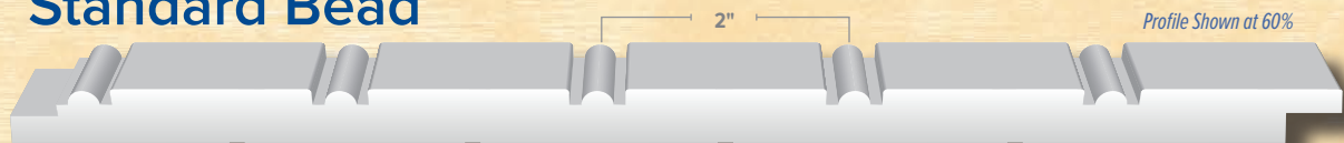
2" STANDARD BEAD (10" FACE) 1 LINEAL FT = .83 SQ FT – ORDER IN 4 PIECE INCREMENTS
